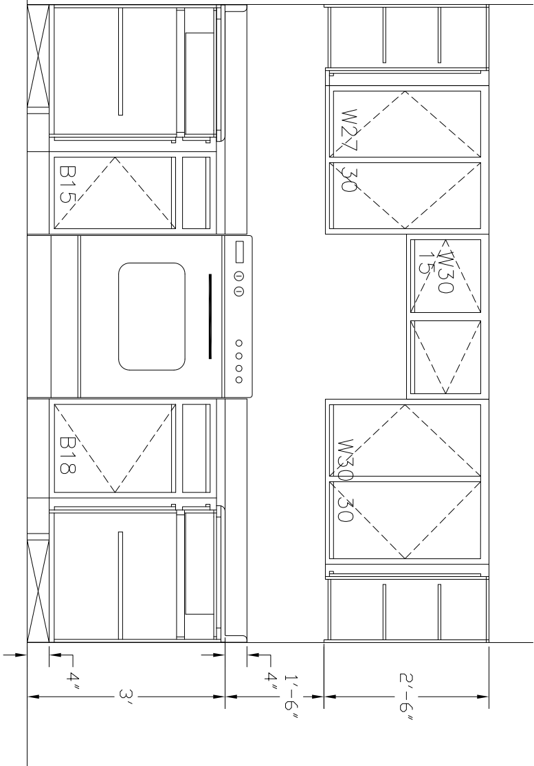
A C9 TYPE "B" UPPER KITCHEN ELEVATION SCALE : 1/2" = 1'
