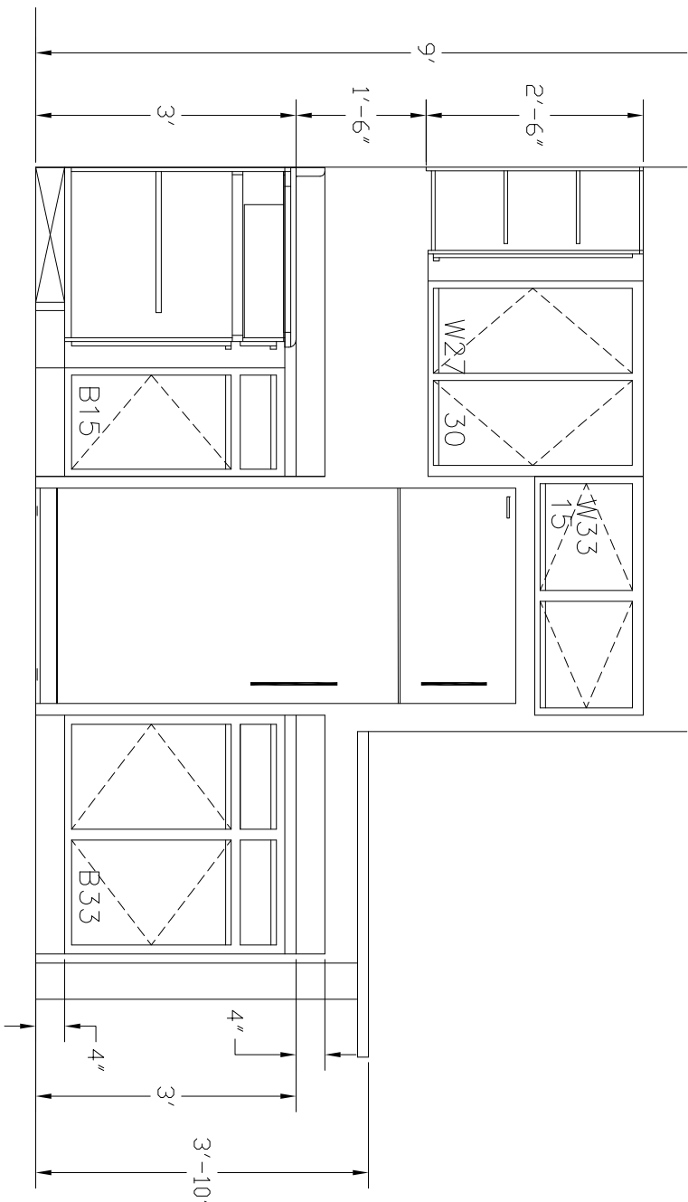
C C9 TYPE "B" UPPER KITCHEN ELEVATION SCALE : 1/2" = 1'
