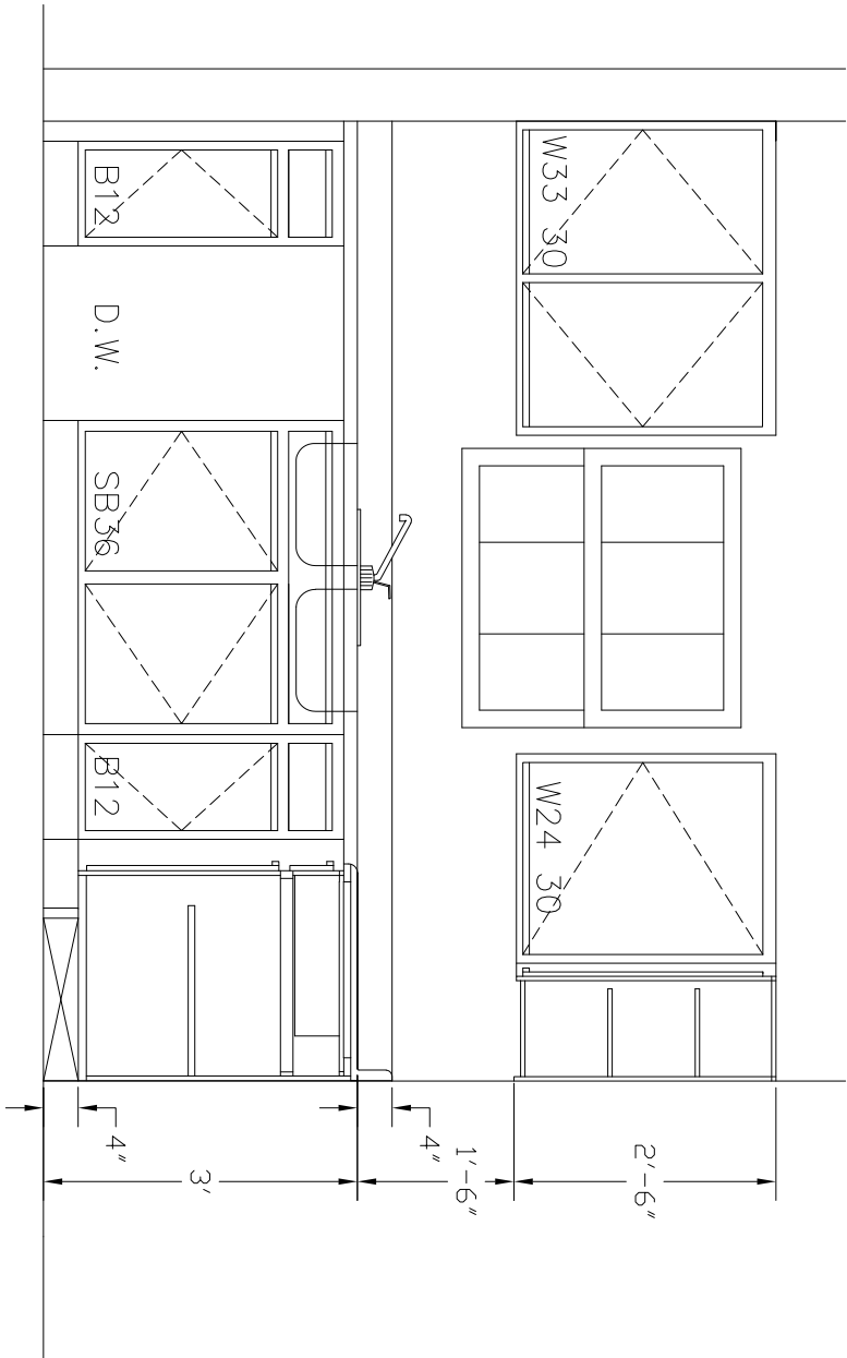
B C9 TYPE "B" UPPER KITCHEN ELEVATION SCALE : 1/2" = 1'
