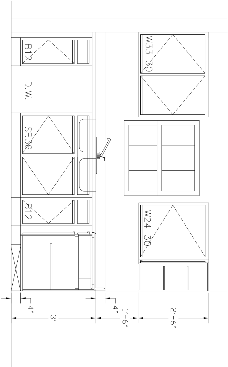
B TYPE “B” LOWER KITCHEN ELEVATION C8 SCALE : 1/2" = 1'
