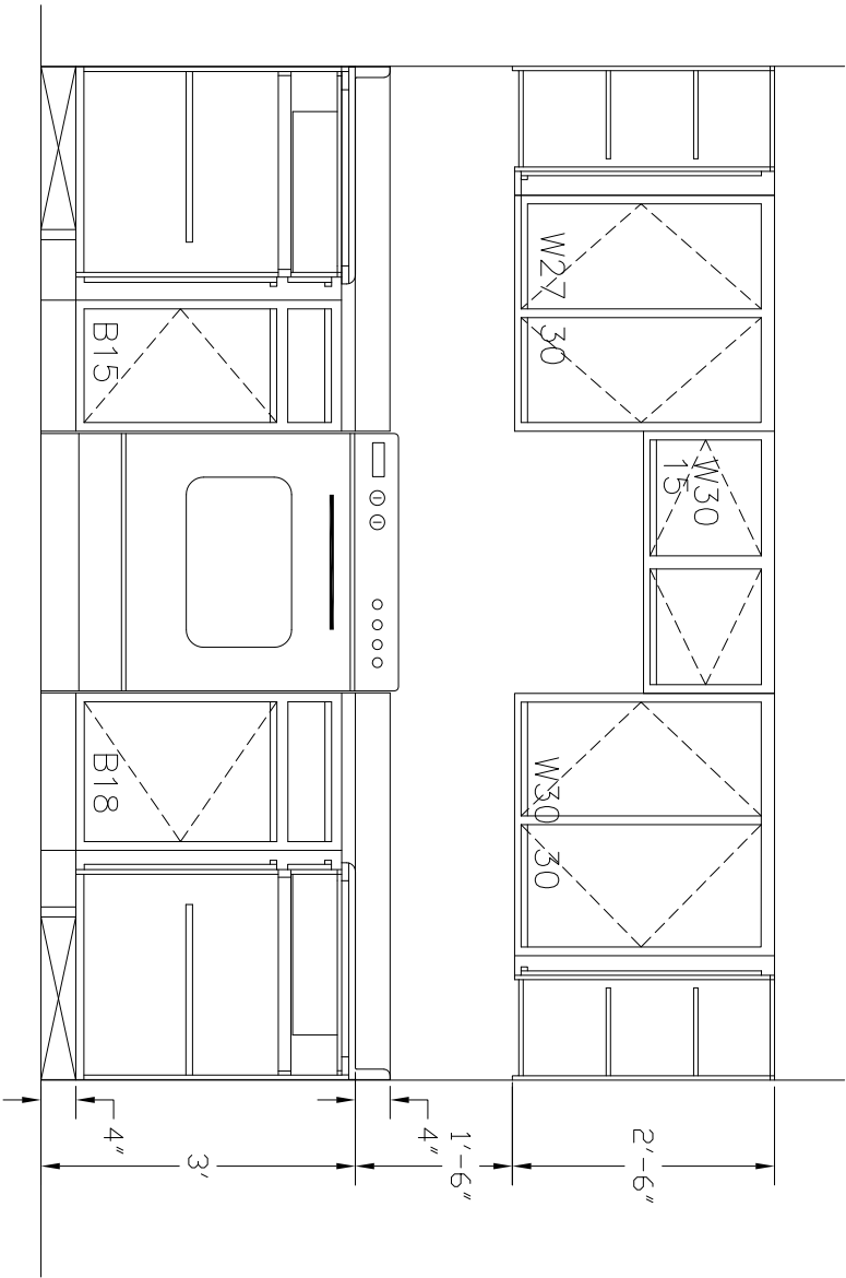
A TPE “B” LOWER KITCHEN ELEVATION C8 SCALE : 1/2" = 1'
